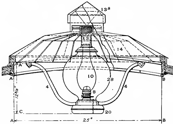
Fig. 3308. Sectional View. STREET-CAR CENTER-LAMP.
